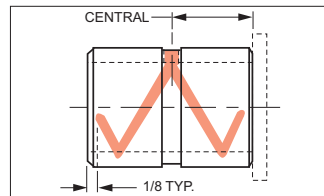
STYLE AJ: With oil groove and hole. Does not break out.
