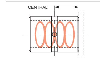
STYLE AY: With oil groove and hole. Double figure eight.
