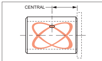
STYLE AU: With oil hole. Double loop.
