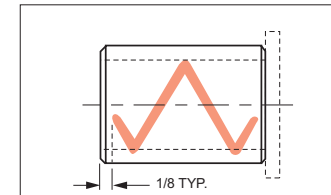
STYLE AF: Does not break out on either end.
