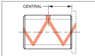
STYLE AB: With oil hole. Breaks out on both ends.
