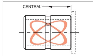
STYLE AV: With oil groove and hole. Double loop.
