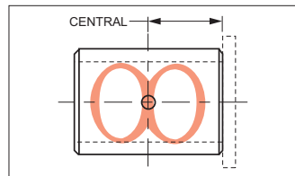
STYLE AN: With oil hole. Figure eight.
