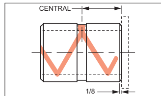
STYLE AG: With oil groove and hole. Breaks out on bottom end.
