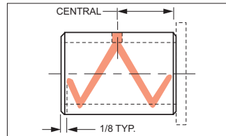
STYLE AC: With oil hole. Does not break out on either end.
