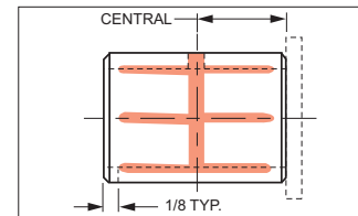
STYLE AL: With oil hole. Does not break out.
