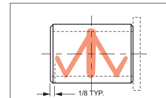
STYLE AM: Does not break out. With I.D. groove.
