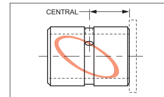
STYLE AS: With oil groove and hole. Single Loop.
