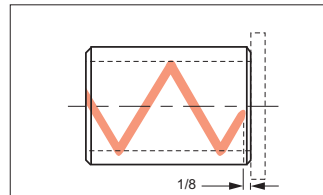
STYLE AD: Breaks out bottom end only.
